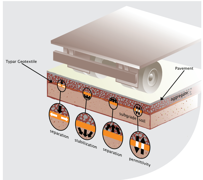
TYPAR stabilizes and preserves paved roads by providing a separation layer between the aggregate base and subgrade.
