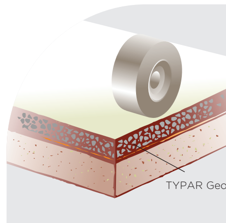
With TYPAR, aggregate won't sink into base soil but stays intact to support loads.
