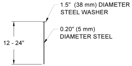
Figure 6: Securing Pin
