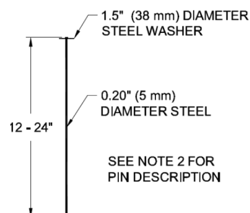
Figure 4: Securing Pin
