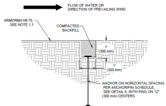
Figure 3: Terminal Channel (TC) Figure Trench
