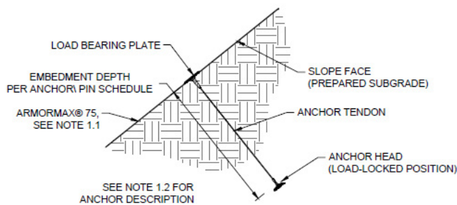
Figure 20: Anchor Detail
