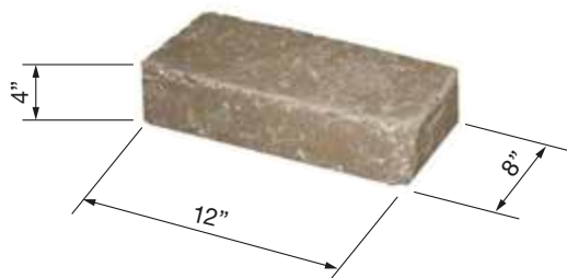
Stone Wall II™ Dimensions
